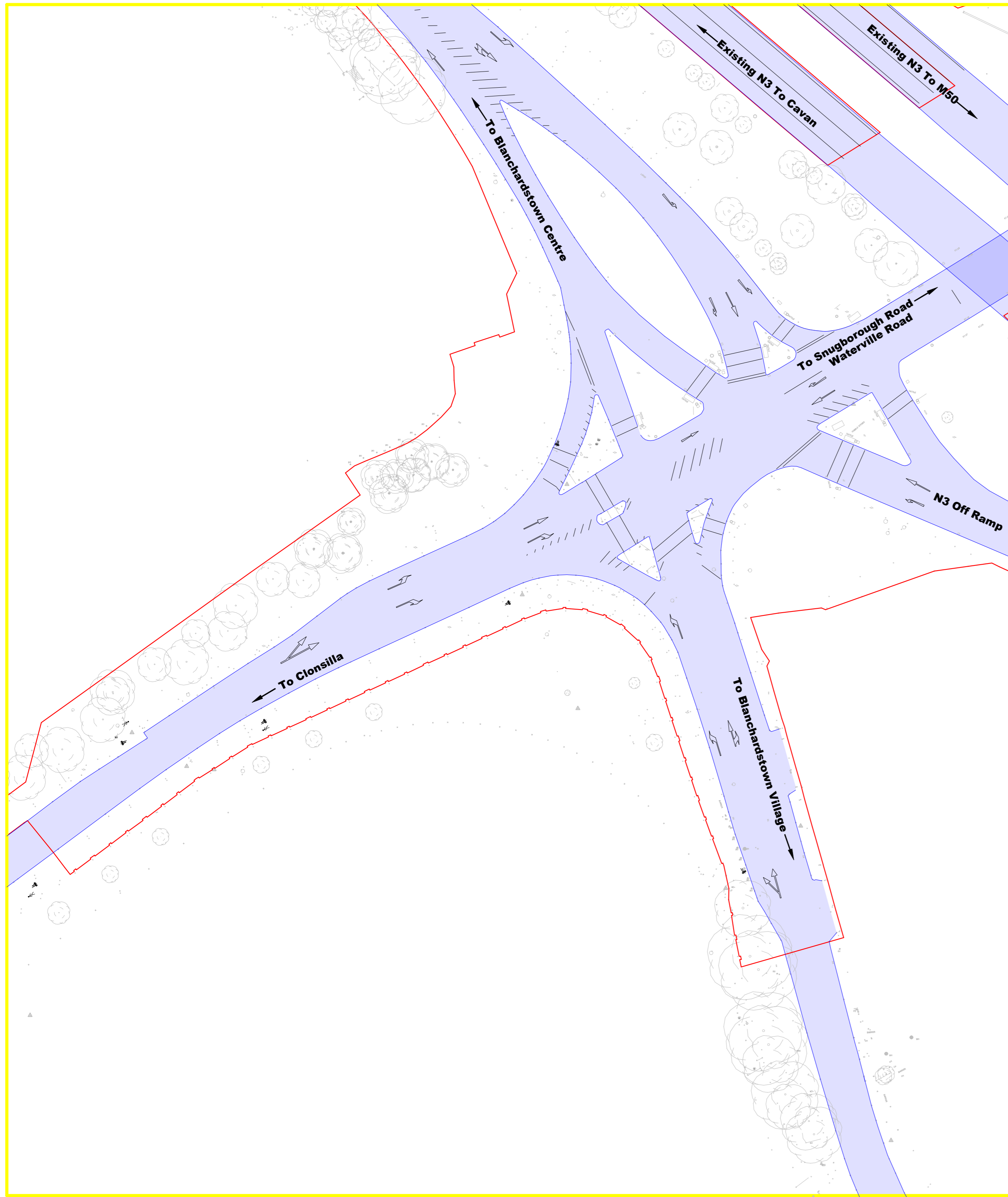
A3 EXISTING SNUGBOROUGH ROAD JUNCTION
