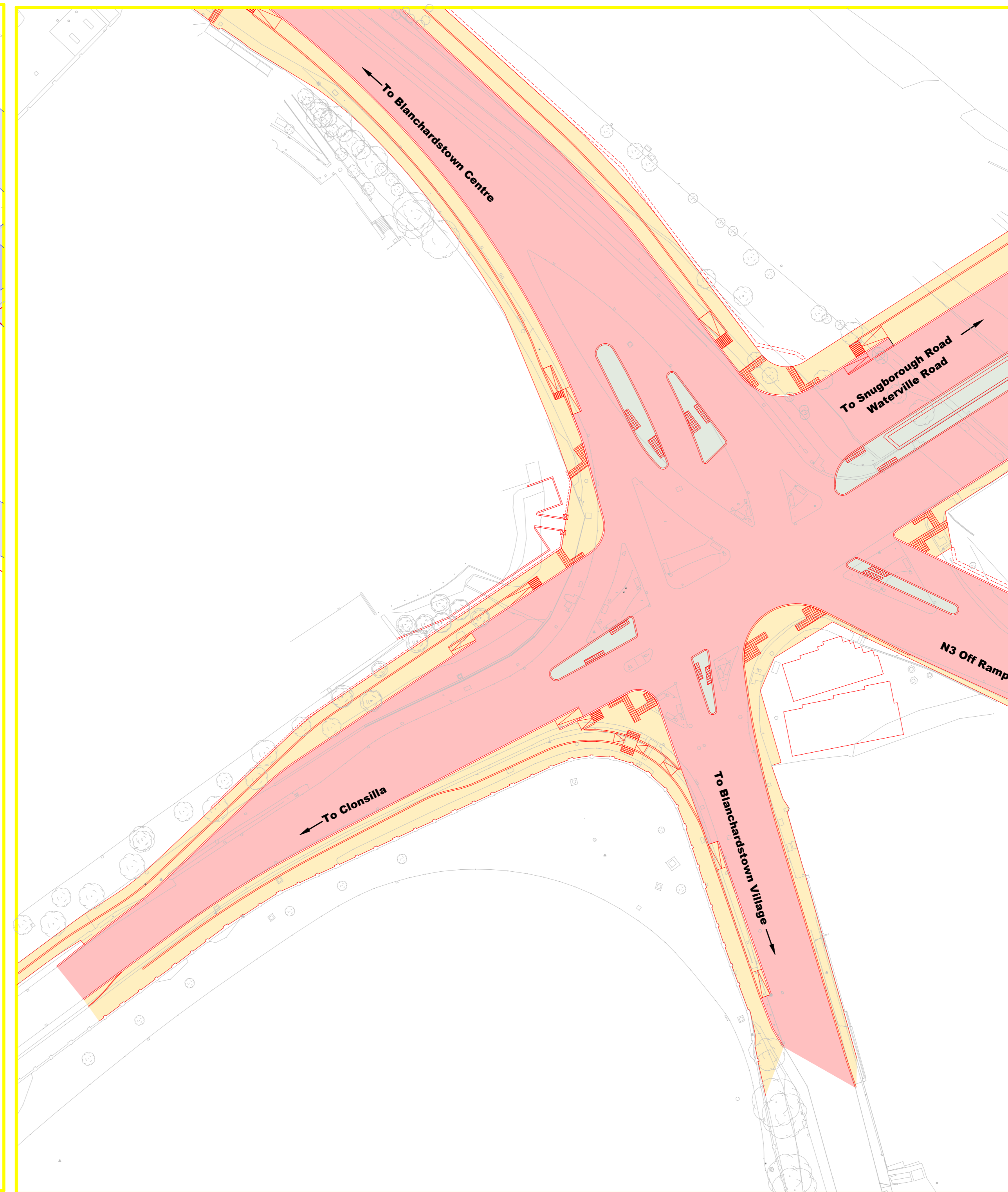
A3 PROPOSED SNUGBOROUGH ROAD JUNCTION
